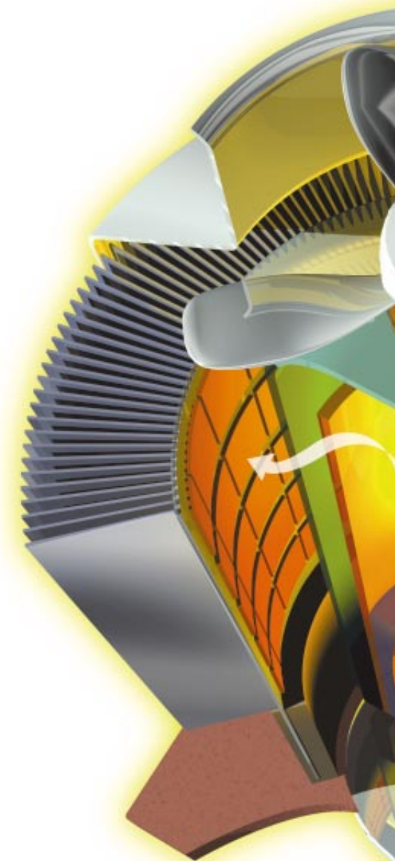
THERMOPHOTOVOLTAIC GENERATOR turns radiant heat into electricity. The burner ( center ) generates heat, whose infrared photons hit a radiator ( green enclosure ). The radiator channels certain infrared wavelengths to arrays of photovoltaic cells ( grid ) that convert the energy to electricity.
